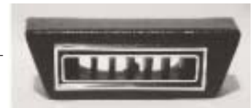
63016-VUL Double louver assembly 11 3/8" x 2 1/2". For 2 1/2" hose. 63316-VUL (all black)
